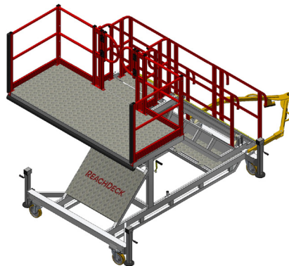
211103 ReachDeck Platform (Large) 1.0mL - 2.5mW with Standard Guardrail Frames
