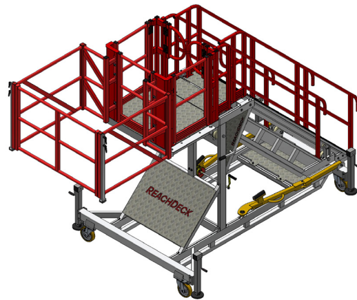
210378 ReachDeck with 1.5mW Loop Guardrail Attachment
