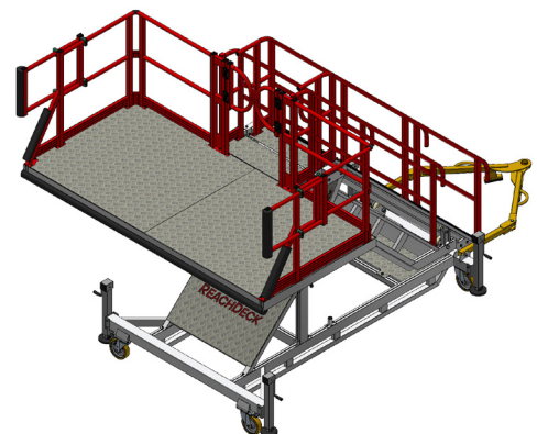
211104 ReachDeck Platform (XL) 2.4mL - 3.0mW with Standard Guardrail Frames
