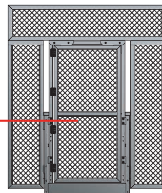
ENTRY/EXIT SWING GATE WITH MESH
