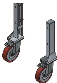
BOLT-ON CASTORS AND BRACKETS
