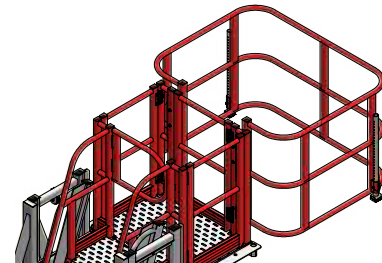
210378 Small Loop Guardrail Frame
