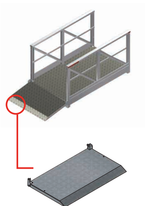
HINGING END RAMP 210135
