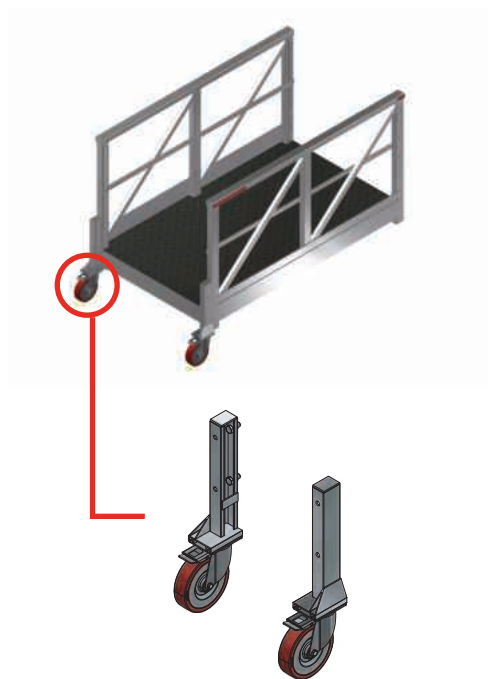
BOLT-ON CASTORS AND BRACKETS 210138
