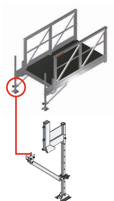
BOLT-ON HEIGHT ADJUSTABLE BRACKETS 210139
